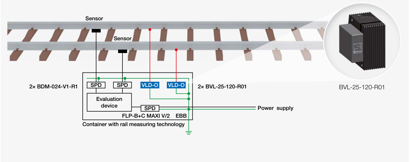
Fig. 6 Installation of VLD class 2.2 for potential equalizing between return circuit and technology's equipotential bounding bar
