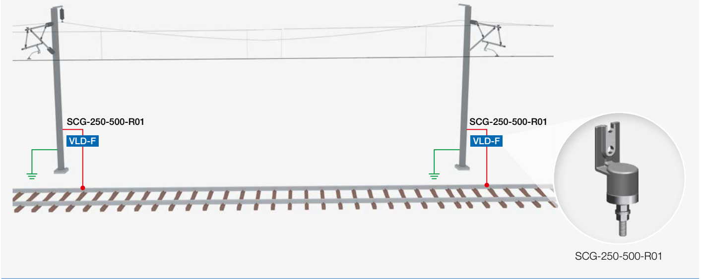
Fig. 5 Installation of VLD class 2.2 and VLD class 1 at railway and switching station according to EN 50526-3
