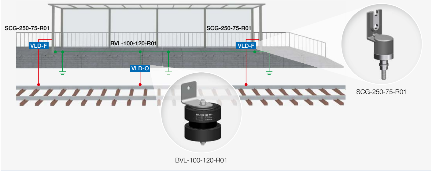
Fig. 6 Installation of VLD class 2.2 for potential equalizing between return circuit and technology's equipotential bounding bar
